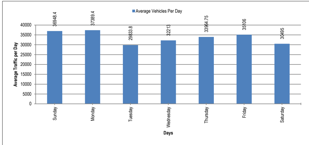
Figure 2-6: Weekly Trend of Traffic at Jhelum (N-5)
