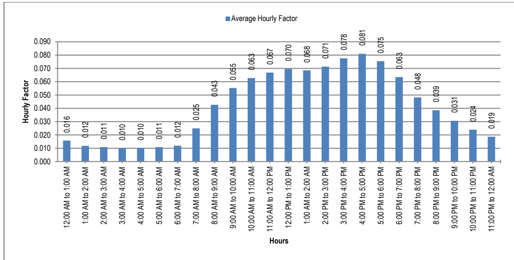
Figure 2-7: Hourly Factor at Jhelum (N-5)
