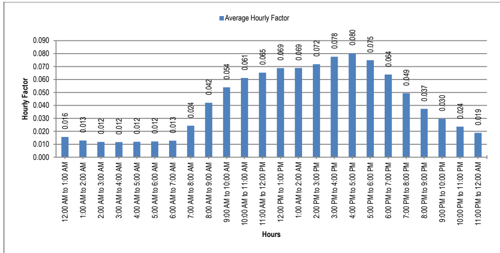
Figure 4-7: Hourly Factor at Pattoki (N-5)
