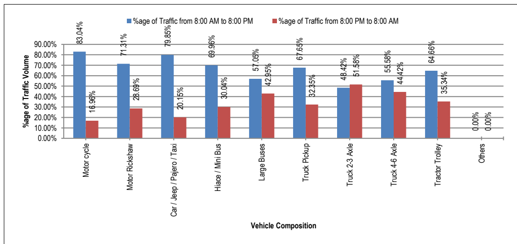
Figure 7-8: Percentage of Traffic Composition in Day and Night Time at Khairpur (N-5)
