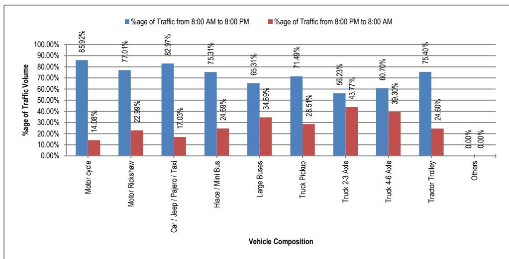
Figure 3-8: Percentage of Traffic Composition in Day and Night Time at Kamoke (N-5)
