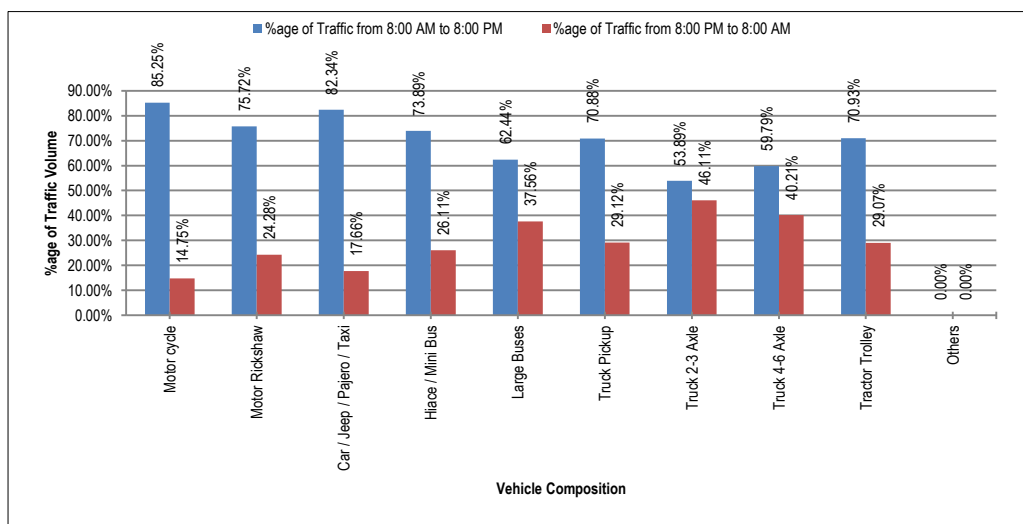
Figure 4-8: Percentage of Traffic Composition in Day and Night Time at Pattoki (N-5)
