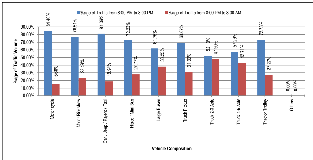
Figure 2-8: Percentage of Traffic Composition in Day and Night Time at Jhelum (N-5)
