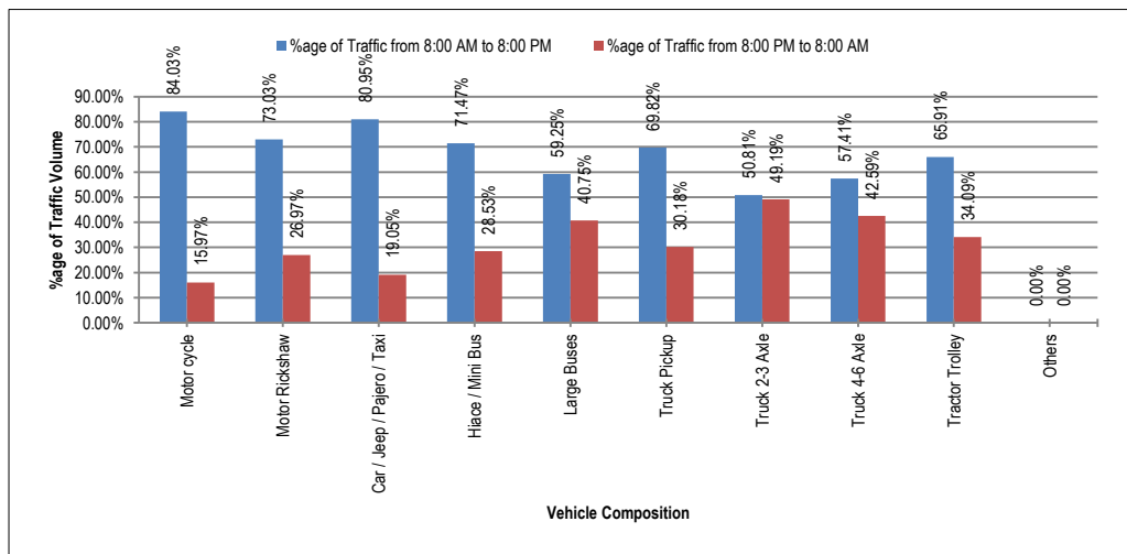
Figure 6-8: Percentage of Traffic Composition in Day and Night Time at Sadiqabad (N-5)
