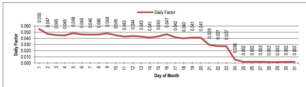
Figure 4-2: Daily Traffic Factor at Pattoki (N-5)
